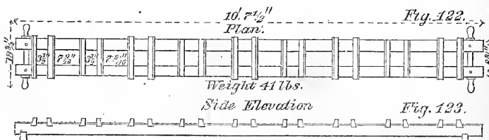
Pontoon Saddle.
